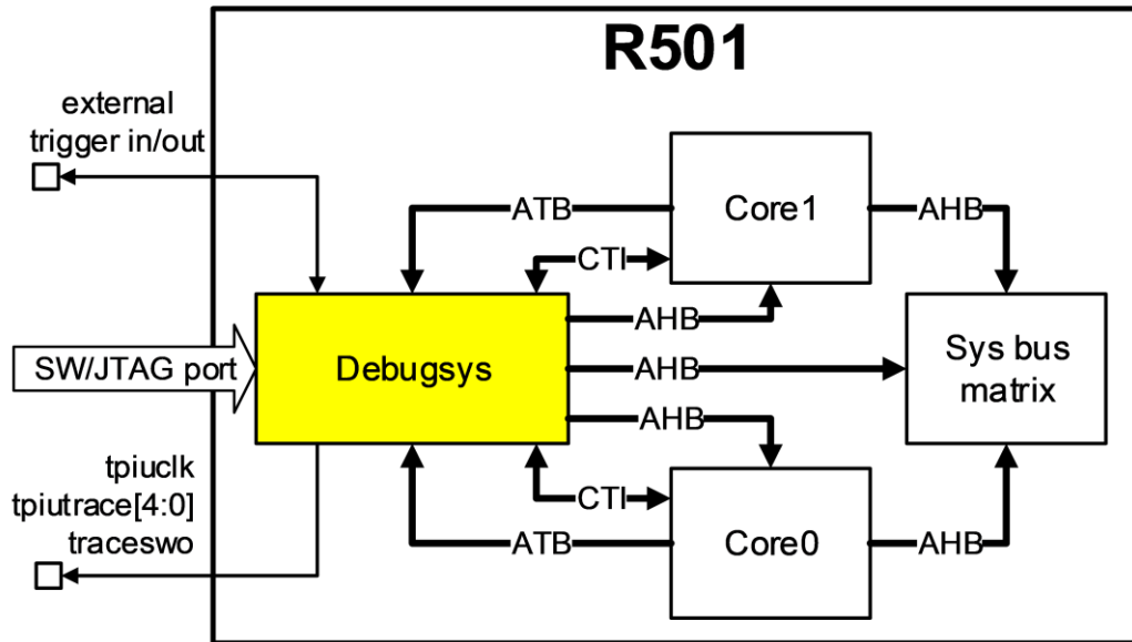
Figure 5 Typical Integration of Debug System
