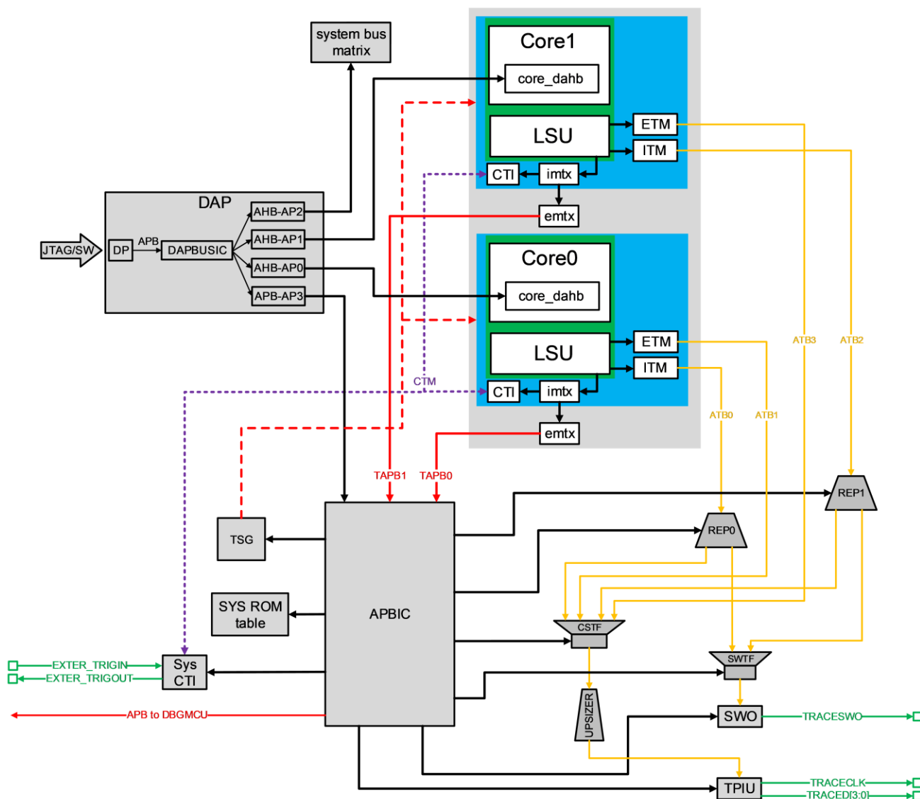
Figure 4 Structure Block Diagram
