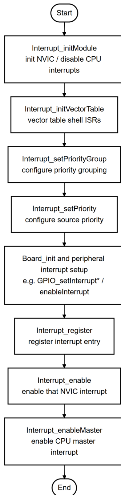
Figure 3 Interrupt initialization flow
